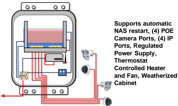
At the edge IP Video via 3G Cellular Includes 2 TB Storage, Modem, Switch
