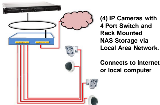
IP Networked Camera with Networked Storage System
