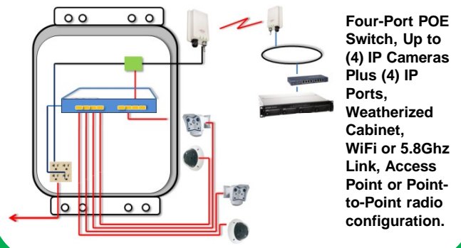
IP Video via WiFi or 5.8GHz Link. Storage at the Network side
